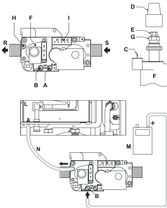
fig. 26 - Valvola gas
