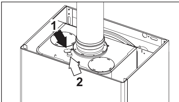
fig. 28 - Analisi fumi DIVAtop MICRO LN F 24
