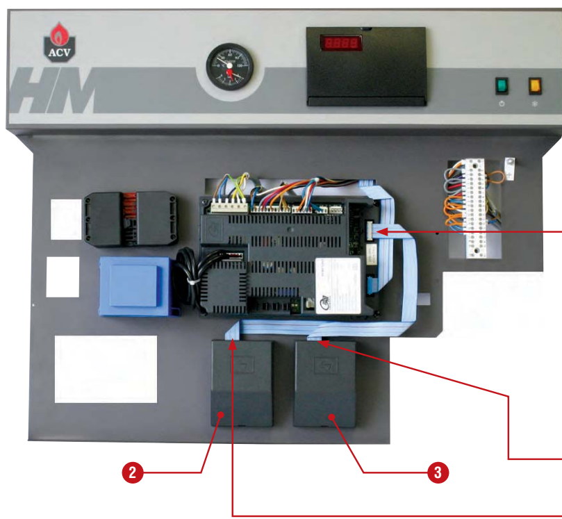
Pannello HeatMaster® 71 / 101
