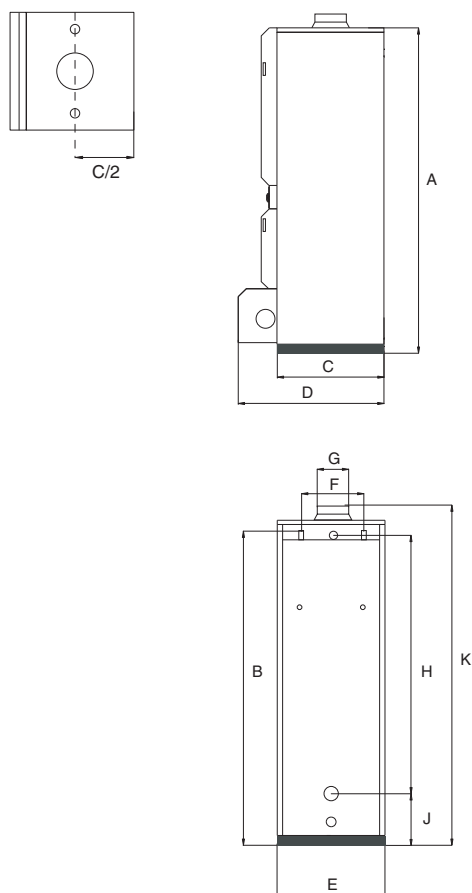
HeatMaster® 71 - 101
