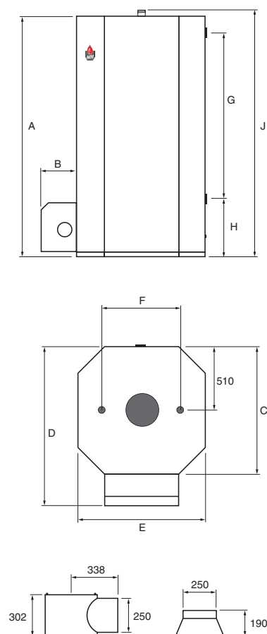
HeatMaster® 201
